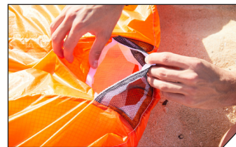
10 Open the Leading Edge air intake velcro to access valve.
