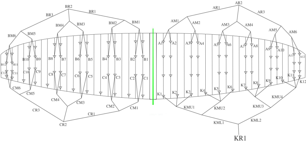
R1 V2 - 6M/7M RIGGING DIAGRAM
