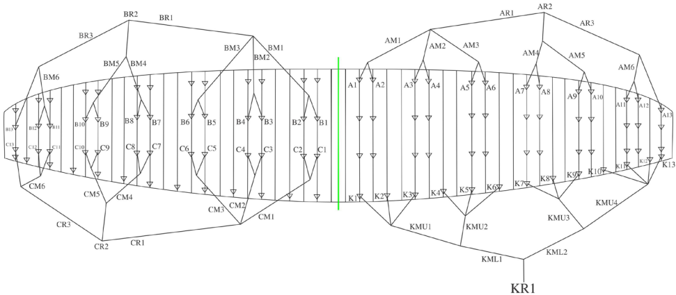
R1 V2 - 8M/9M RIGGING DIAGRAM
