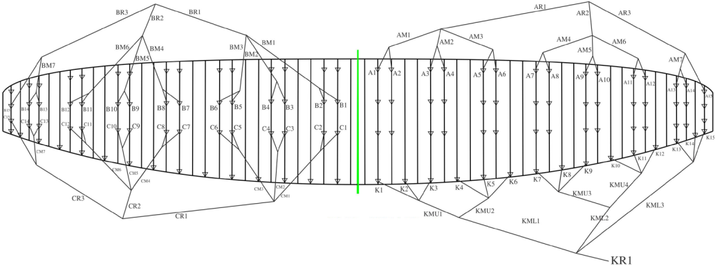
R1 V2 - 15M/17M/18M/19M/21M RIGGING DIAGRAM
