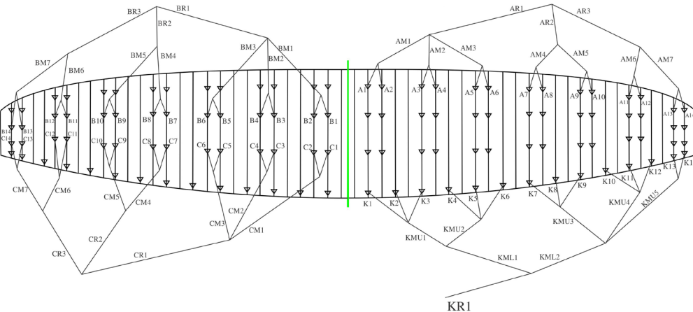
R1 V2 - 10M/11M/13M RIGGING DIAGRAM
