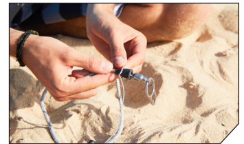
2 Pull the Flag Out Line and connected flying line no.5 out through the Quick Release.
